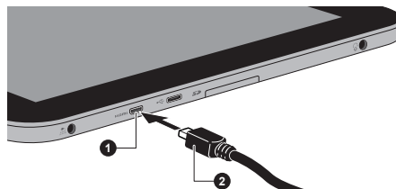
Figure 7-2 Connecting an HDMI cable
